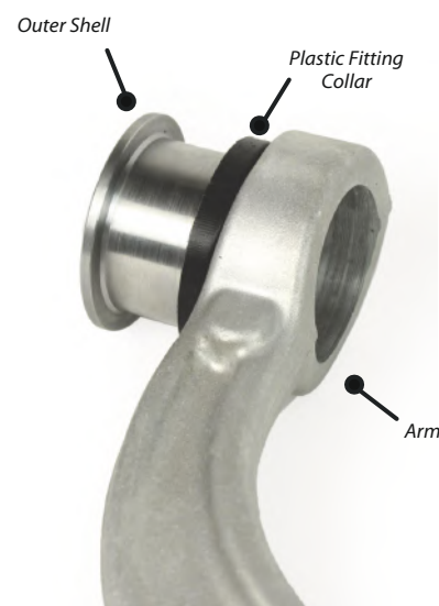
Figure 1 - Orientation of Fitting Collar, for pressing the Rear Bush
